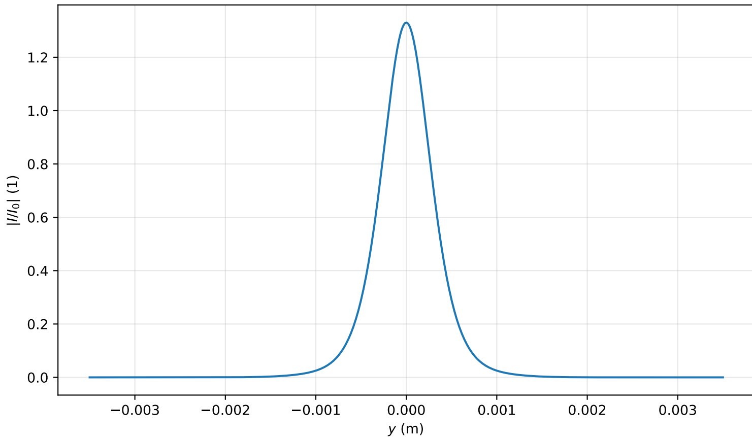
Intensity profile I(x=0, y, z=1.911)/I_0 , P_{in}=0.8P_{cr} , artificial time
